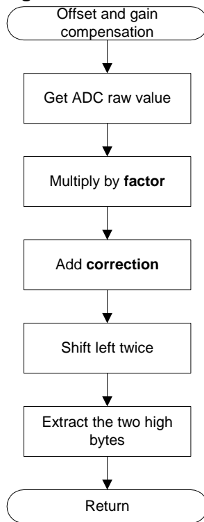
Figure 12. Flowchart for offset and gain compensation
